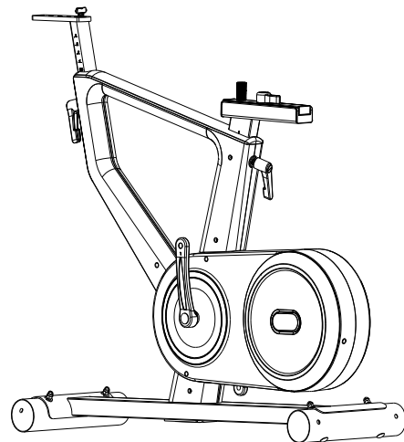
28 MAIN FRAME
